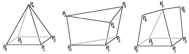
Fig. 32. From left to right: pyramid, wedge, and knife – the only hybrid elements listed in the Verdict Library, a popular reference for the computation of quality metrics of finite elements. Image from [Stimpson et al. 2007].
