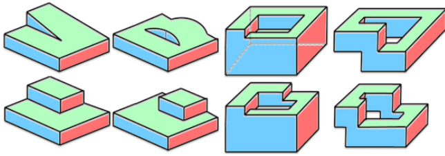
Fig. 17. Top: a set of pathological shapes having sharp creases and surface normals that push polycube deformation energies towards the generation of globally inconsistent orthogonal polyhedra. Bottom: the associated polycubes. Additional corners were strategically introduced to define topologically sound global structures. Image from [Sokolov 2016].
