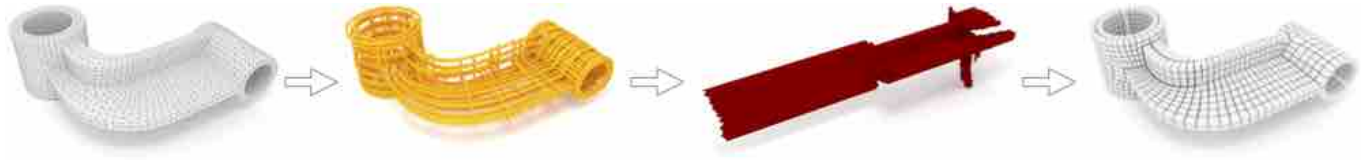
Fig. 19. Frame field based hexahedral mesh generation: Given an input tetrahedral mesh (left), first a boundary aligned and smooth frame field is generated (middle, yellow). The frame field serves as a proxy for the local orientation of hexahedra and thus enables the efficient generation of an integer-grid map (middle, red), which induces a hexahedral mesh (right). Image from [Liu et al. 2018].
