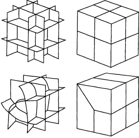
Fig. 4. Two examples (top and bottom) of the relation between dual and primal mesh representation. Left: dual cell complex, formed by an arrangement of 2-manifold sheets. Right: corresponding hexahedral mesh. Image from [Murdoch et al. 1997].
