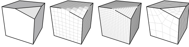
Fig. 8. Incorporating an input feature network (left, bold lines) into the output hex-mesh is not possible if the connectivity does not align to it (middle left), even refining the mesh (middle right). Key to feature preservation is the ability to align surface edges to the input network, carefully positioning mesh singularities (right). Image from [Livesu et al. 2020].
