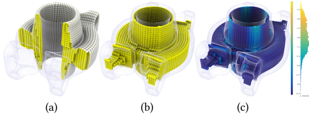
Fig. 33. The interactive visualization tools offered by Hexalab: Internal exploration using a sweeping plane (a) or the peeling tool (b); Coloring elements by their quality and the resulting histogram (c).
