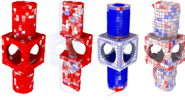
Fig. 30. A degraded hex-mesh obtained by randomly displacing interior vertices (left, first two columns), optimized with a state-of-the-art corner based approach [Aigerman and Lipman 2013]. Hard constraining the surface does not allow to fully untangle the mesh (middle right, see red elements and spikes at the bottom and top). Relaxing it yields a mesh with positive minimum Jacobian, but introduces excessive surface deviation (right). Scaled Jacobian is color coded, from pure red ( SJ \leq 0 ) to pure blue ( SJ = 1 ).
