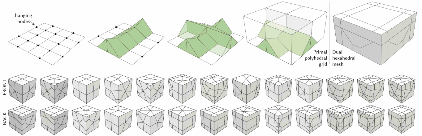
Fig. 12. Dual methods regularize the valence of hanging nodes (black dots) by connecting them pairwise along triangular bridges, so that the dual is a hex-mesh. Top: the flat transition firstly introduced in [Maréchal 2009]. Bottom: the set of atomic schemes introduced in [Livesu et al. 2021] to handle all possible transitions in strongly and weakly balanced grids. Images partly from [Livesu et al. 2021].
