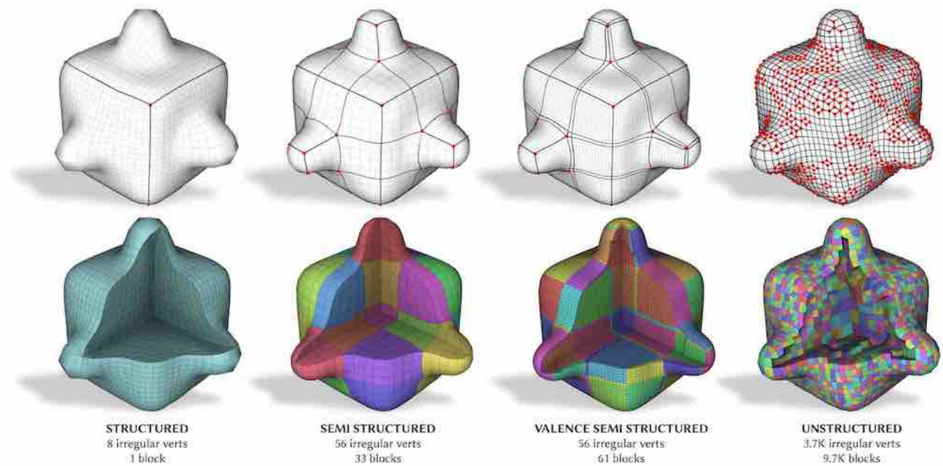
Fig. 1. Hex-meshes can be categorized according to their structural regularity, which depends on the amount of irregular edges and vertices present in the mesh (red dots) and on how they are connected to each other (thick lines). The first three meshes were computed with a polycube method [Livesu et al. 2013], the latter with an octree method [Gao et al. 2019].
