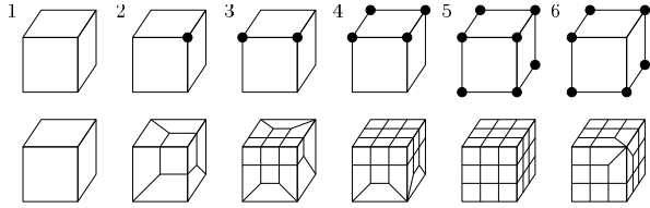
Fig. 13. The set of 6 out of 22 schemes of 3-refinement introduced in [Schneiders 1996b]. The 1 and the 5 are respectively the empty and the fully refined hexahedra, while the other templates are used to manage the transition between them. Image taken from [Schneiders 2000].
